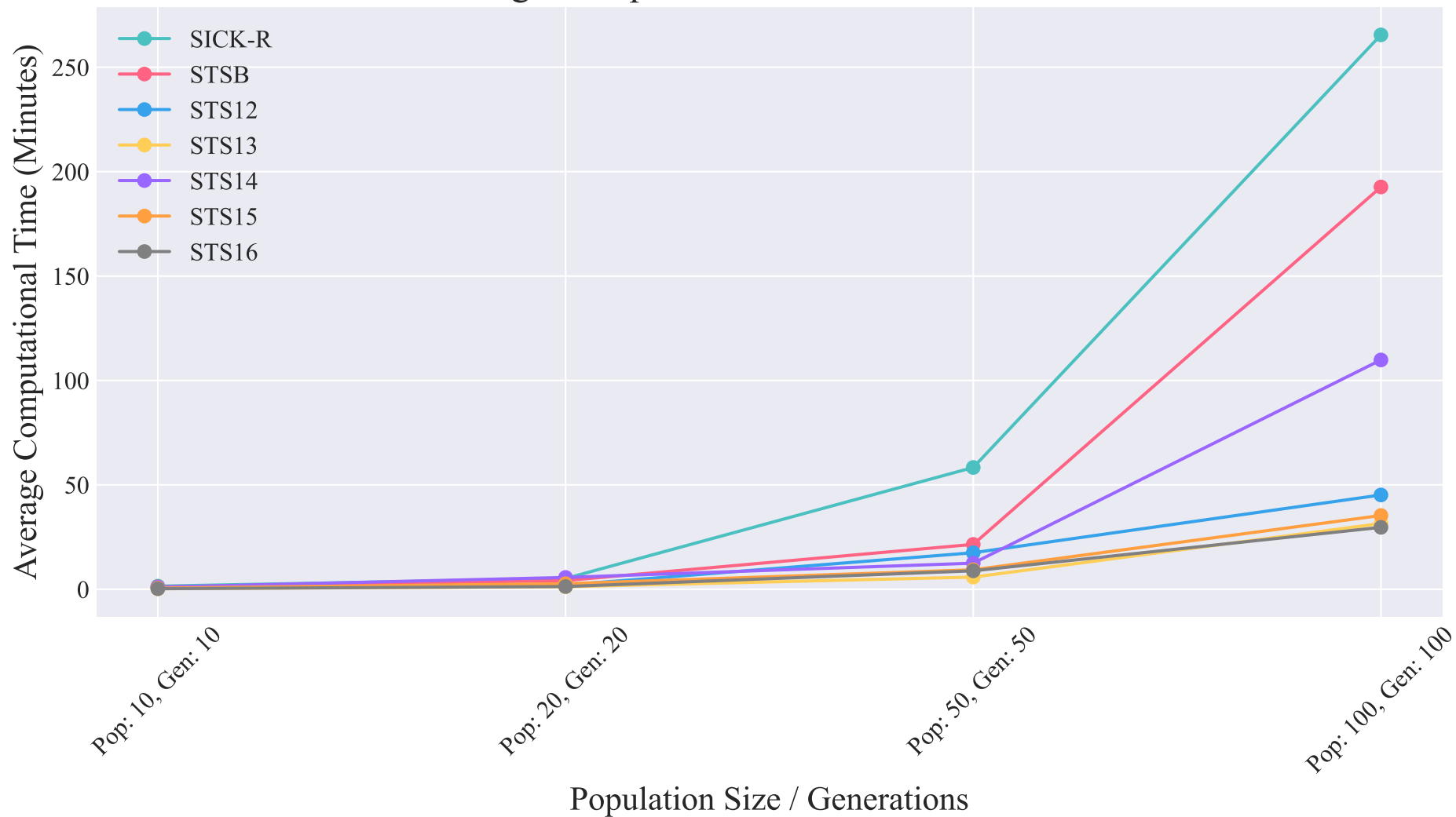
Average Computational Time Across Datasets
